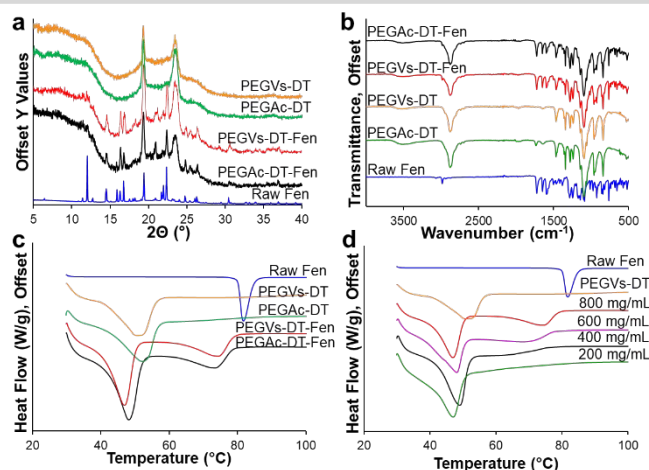
Figure 3. Characterization of Fen crystals in PEG hydrogel matrix. a. PXRD curves of raw Fen crystalline form I, neat PEGVs-DT, PEGAc-DT hydrogel matrices, Fen PEGVs-DT and Fen PEGAc-DT composite micro-hydrogels prepared with 800 mg/mL Fen in anisole, b. FTIR spectra of raw Fen crystalline form I, neat PEGVs-DT, PEGAc-DT hydrogel matrices, Fen PEGVs-DT and Fen PEGAc-DT composite micro-hydrogels prepared with 800 mg/mL Fen in anisole, c. DSC thermograms of raw Fen crystalline form I, neat PEGVs-DT, PEGAc-DT hydrogel matrices, Fen PEGVs-DT and Fen PEGAc-DT composite micro-hydrogels prepared with 800 mg/mL Fen in anisole, d. DSC thermograms of Fen PEGVs-DT micro-hydrogels prepared with varying Fen concentration in the anisole phase (800-200 mg/mL).
