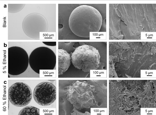
Figure 2. Characterization of Fen morphology in PEG micro-hydrogels. Optical micrographs, surface and cross-section morphology FESEM characterization of a. Blank anisole NE loaded PEGVs-DT micro-hydrogels post cross-linking and solvent exchange in 5 % EtOH anti-solvent sink, b. Fen-anisole NE loaded PEGVs-DT micro-hydrogels after cross-linking and solvent exchange in 5 % EtOH anti-solvent sink and c. Fen-anisole NE loaded PEGVs-DT micro-hydrogels after cross-linking and solvent exchange in 60 % EtOH anti-solvent sink.
