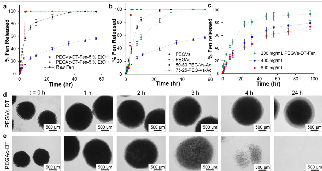
Figure 4. Dissolution of Fen crystals in PEG micro-hydrogel matrix. a. Dissolution profiles of raw Fen in SGF in comparison to the burst release formulation of PEGAc-DT-Fen and the controlled release formulation of PEGVs-DT-Fen, b. Dissolution in SGF of Fen embedded in varying composition of the 4-arm monomers cross-linked with PEG-DT of 100 % PEGVs, 100 % PEGAc, 50-50 PEG-Vs-Ac and 75-25 PEG-Vs-Ac, c. Dissolution in SGF of Fen embedded in PEGVs-DT micro-hydrogels prepared with varying Fen concentration in the anisole phase (800-200 mg/mL), d. Optical micrographs of PEGVs-DT-Fen micro-hydrogels subjected to Fen dissolution in SGF from 0-24 h time points, e. Optical micrographs of PEGAc-DT-Fen micro-hydrogels subjected to Fen dissolution in SGF from 0-24 h time points.
